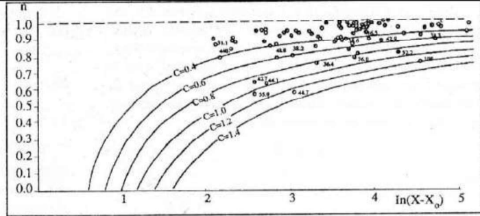
Figure 2 : Graphe de la relation n = f[\ln(X - X_0)] de la r. Touapsé - v. Touapsé, F = 351 \text{ km}^2 , N = 83 crues.
