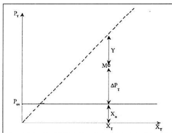
Figure 1 : Graphique de la relation P_T = f(X_T) .
