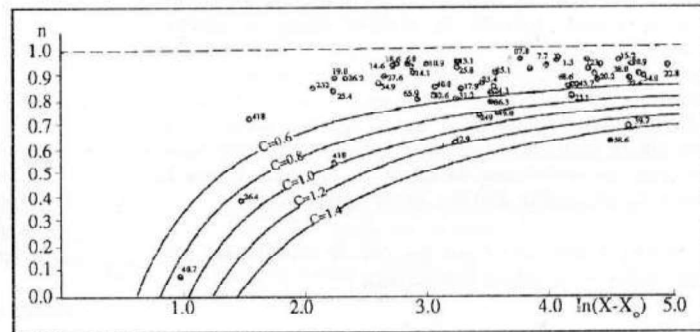
Figure 4 : Graphe de la relation n = f[\ln(X - X_0)] de la r. Kouapsé - Momédovo Chel, F = 14.6 \text{ km}^2 , N = 58 crues.
