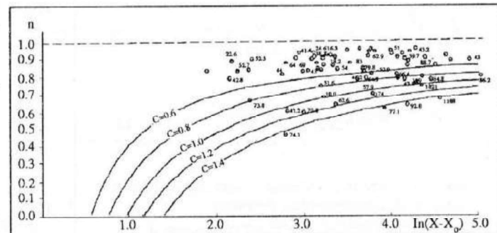
Figure 5 : Graphe de la relation n = f[\ln(X - X_0)] de la r. Psézouapsé - v. Tatianovo, F = 255 \text{ km}^2 , N = 76 crues.
